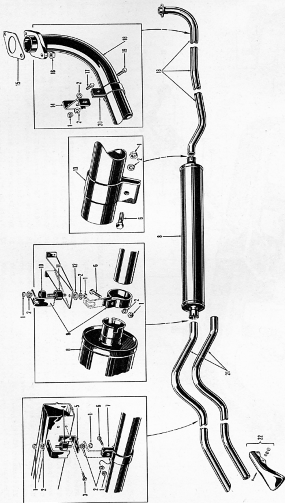
FIGURE 5-2—EXHAUST SYSTEM - EXPLODED VIEW
