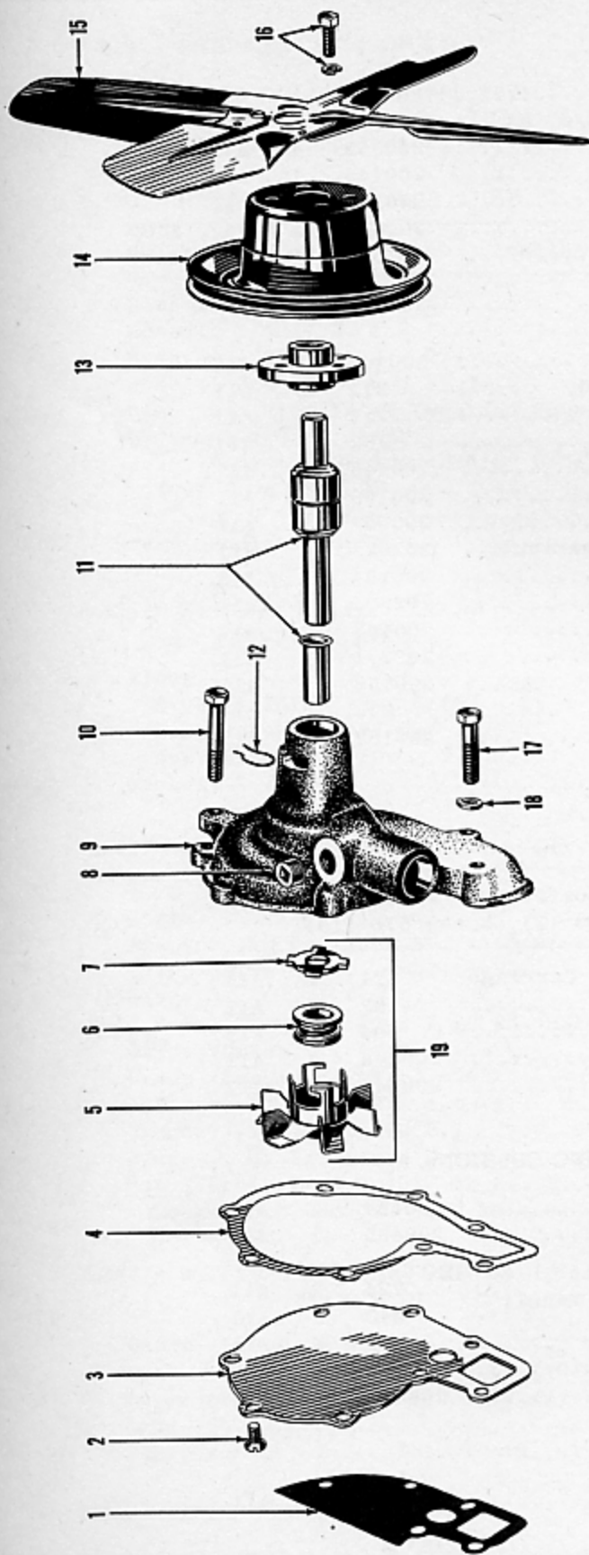
FIGURE 6-1—WATER PUMP - EXPLODED VIEW
