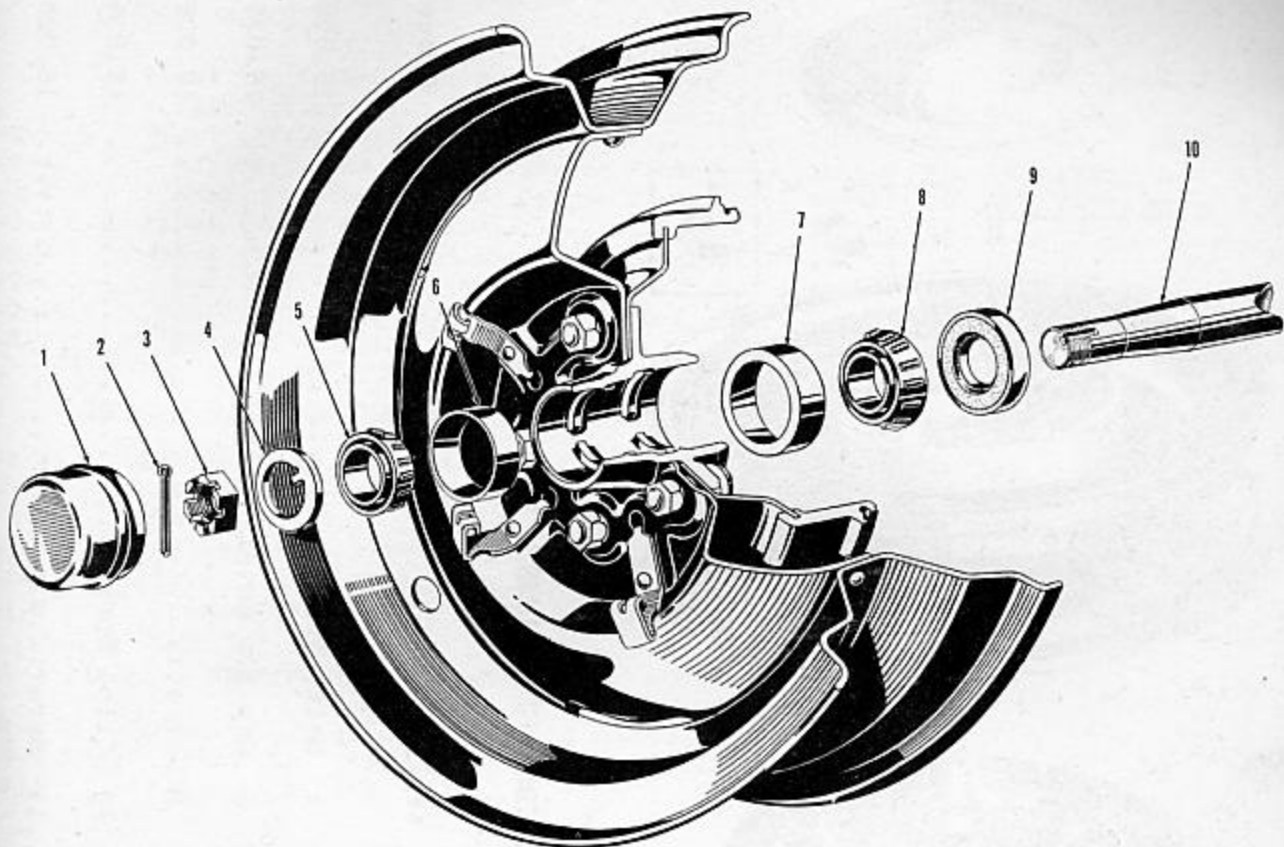
FIGURE 16-1—TYPICAL FRONT WHEEL AND BEARINGS - EXPLODED VIEW
