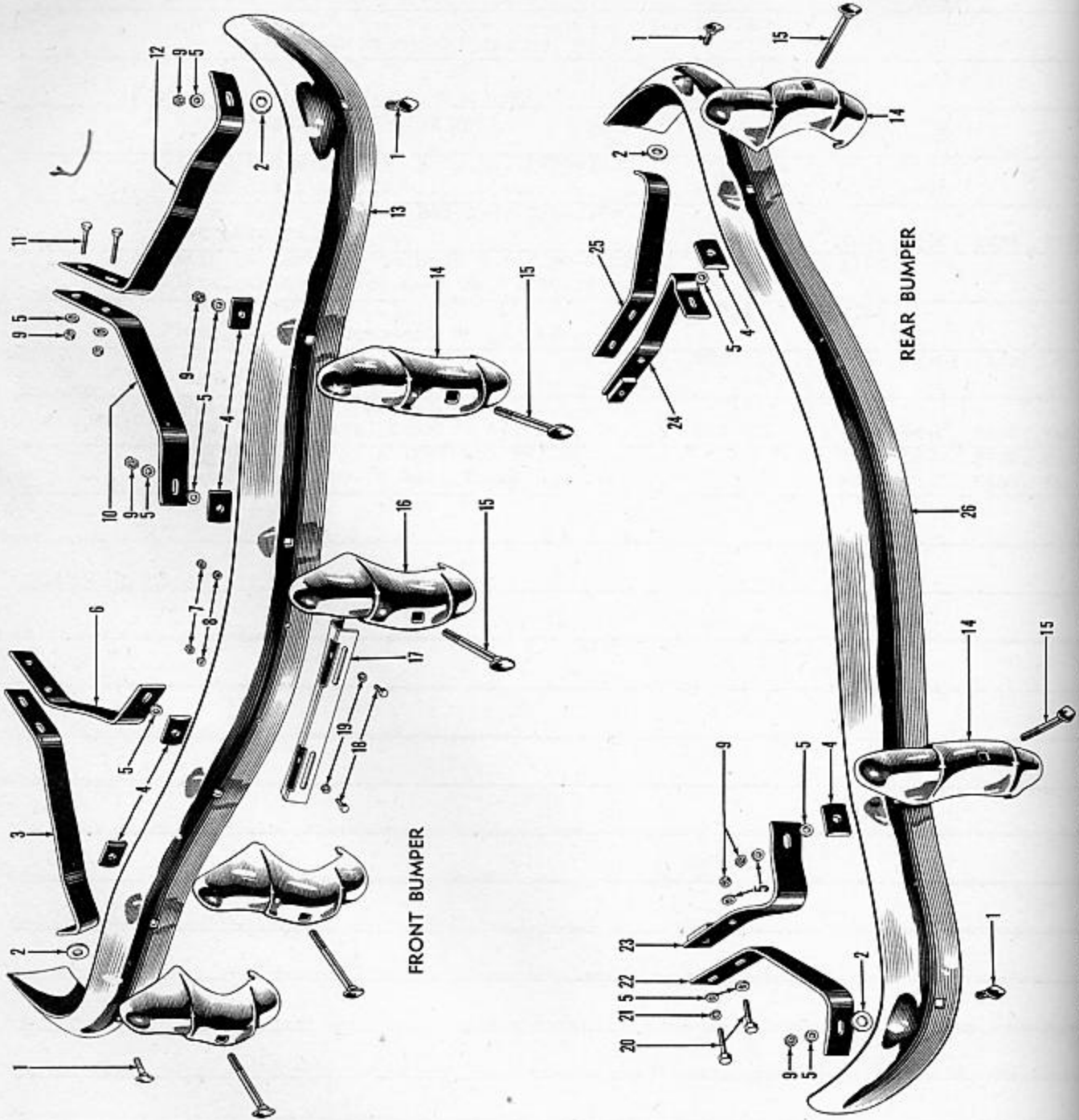
FIGURE 20-1—ONE PIECE FRONT AND REAR BUMPERS - KAISER - EXPLODED VIEW
