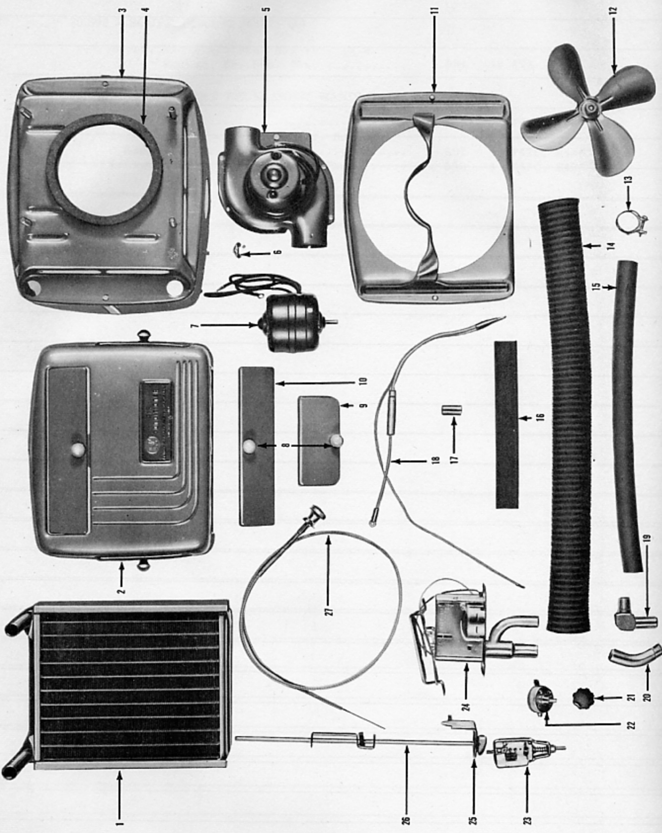
FIGURE 40-1—AIR CONDITIONER - EXPLODED VIEW
