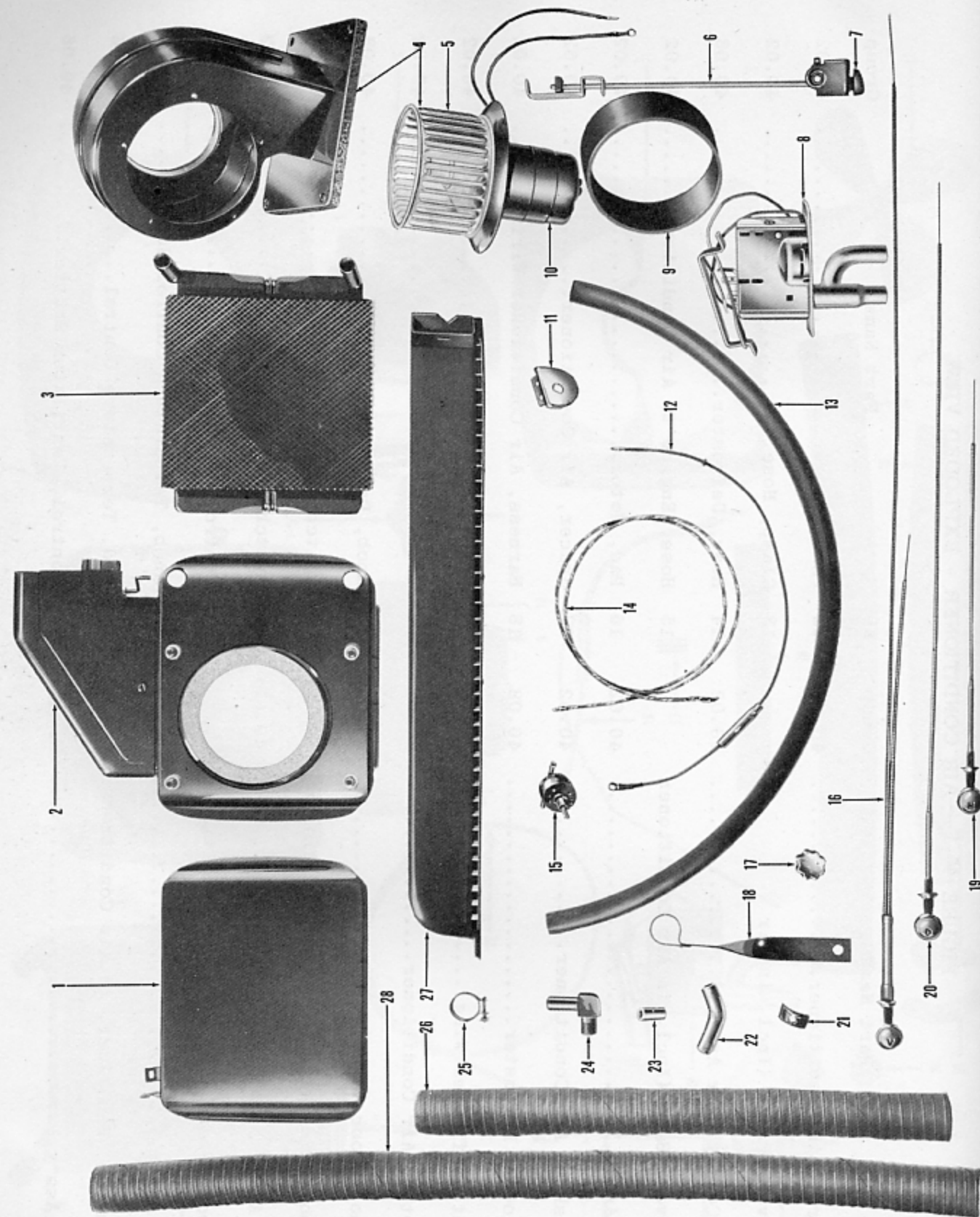
FIGURE 40-2—AIR CONDITIONER - MANHATTAN ONLY - EXPLODED VIEW
