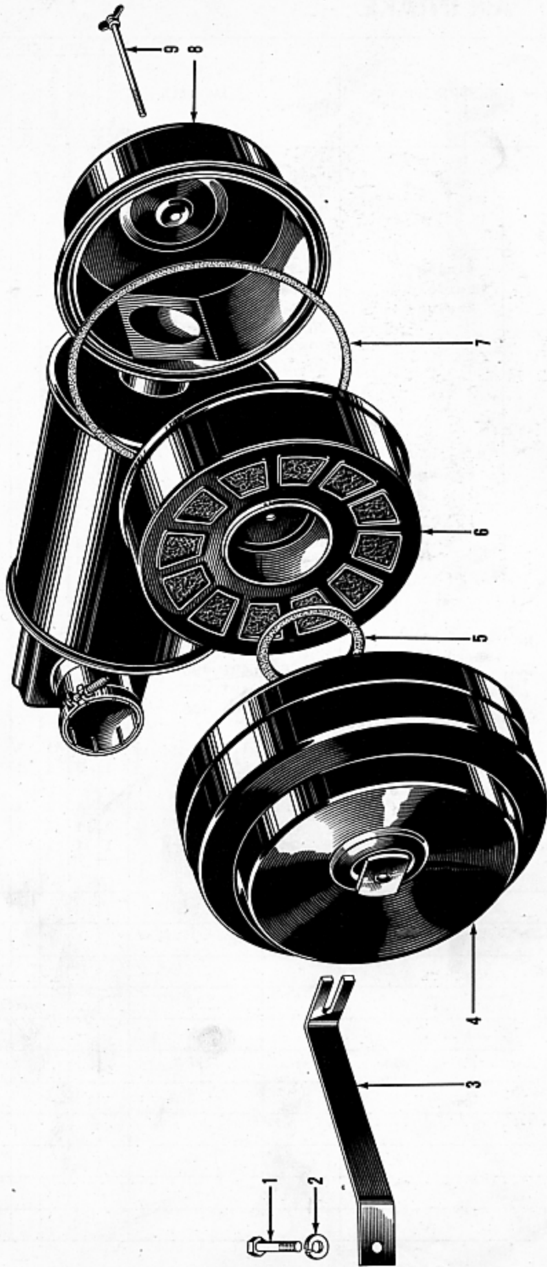
FIGURE 4-2 — AIR CLEANER - DUAL MANIFOLD - ELBOW TYPE - EXPLODED VIEW
