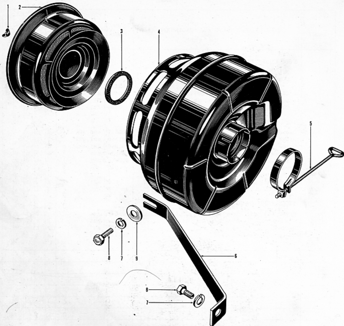
FIGURE 4-1 — AIR CLEANER - DUAL MANIFOLD - EXPLODED VIEW
