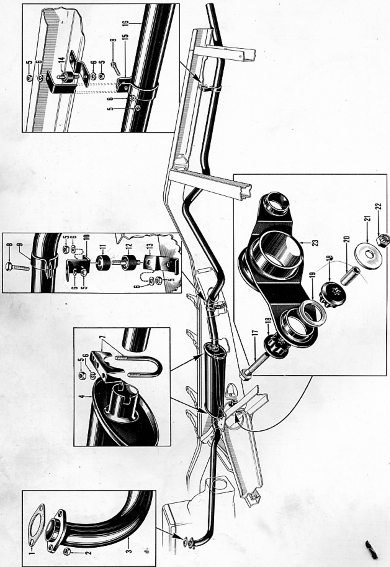
FIGURE 5-2 — EXHAUST SYSTEM AND PROPELLER SHAFT SUPPORT - CONVERTIBLE MODELS
