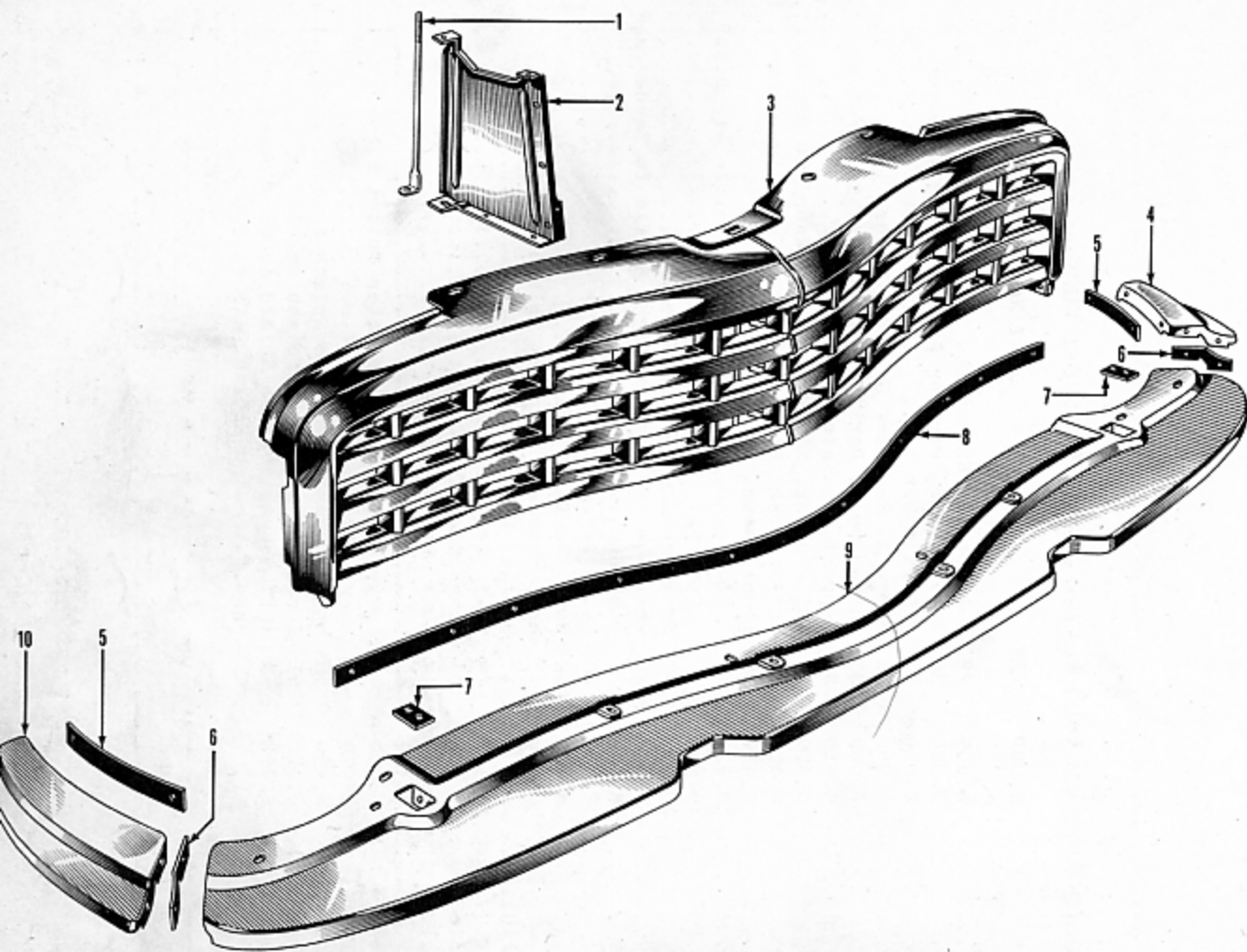
FIGURE 6-3 — FRAZER GRILLE AND FRONT STONE DEFLECTOR
