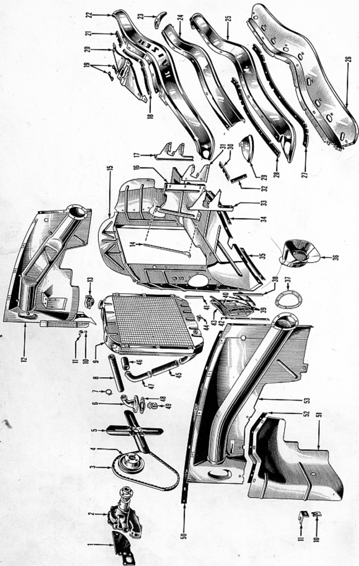
FIGURE 6-2 — COOLING SYSTEM AND RELATED PARTS - EXPLODED VIEW
