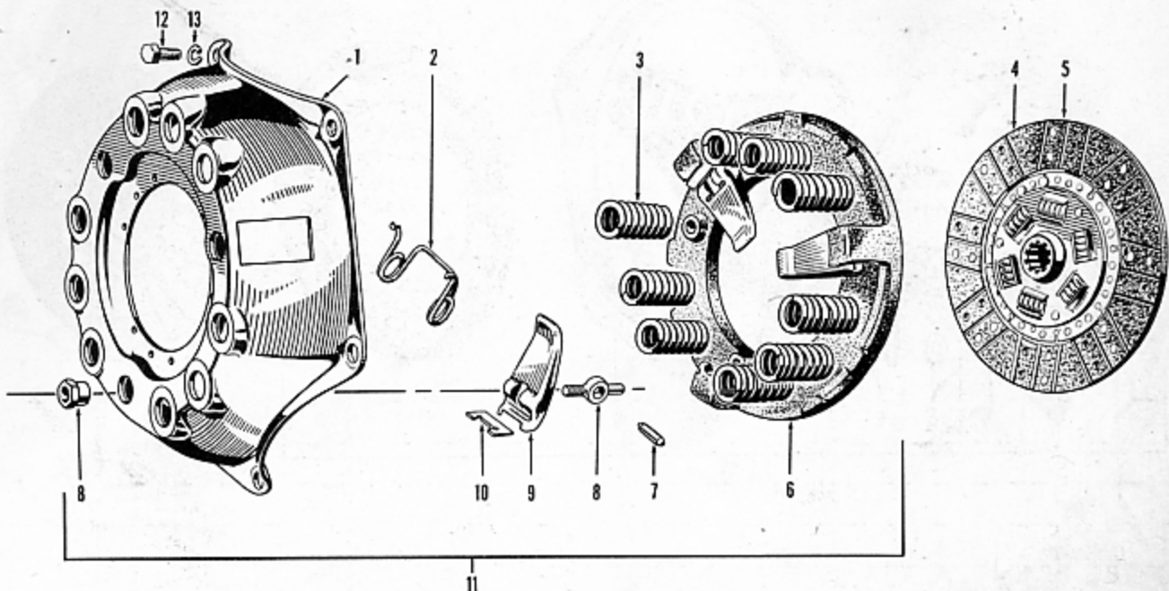
FIGURE 8-1 — TYPICAL CLUTCH -9 SPRING - EXPLODED VIEW
