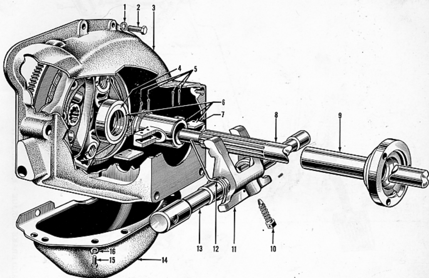
FIGURE 8-3 — CLUTCH RELEASE MECHANISM - EXPLODED VIEW
