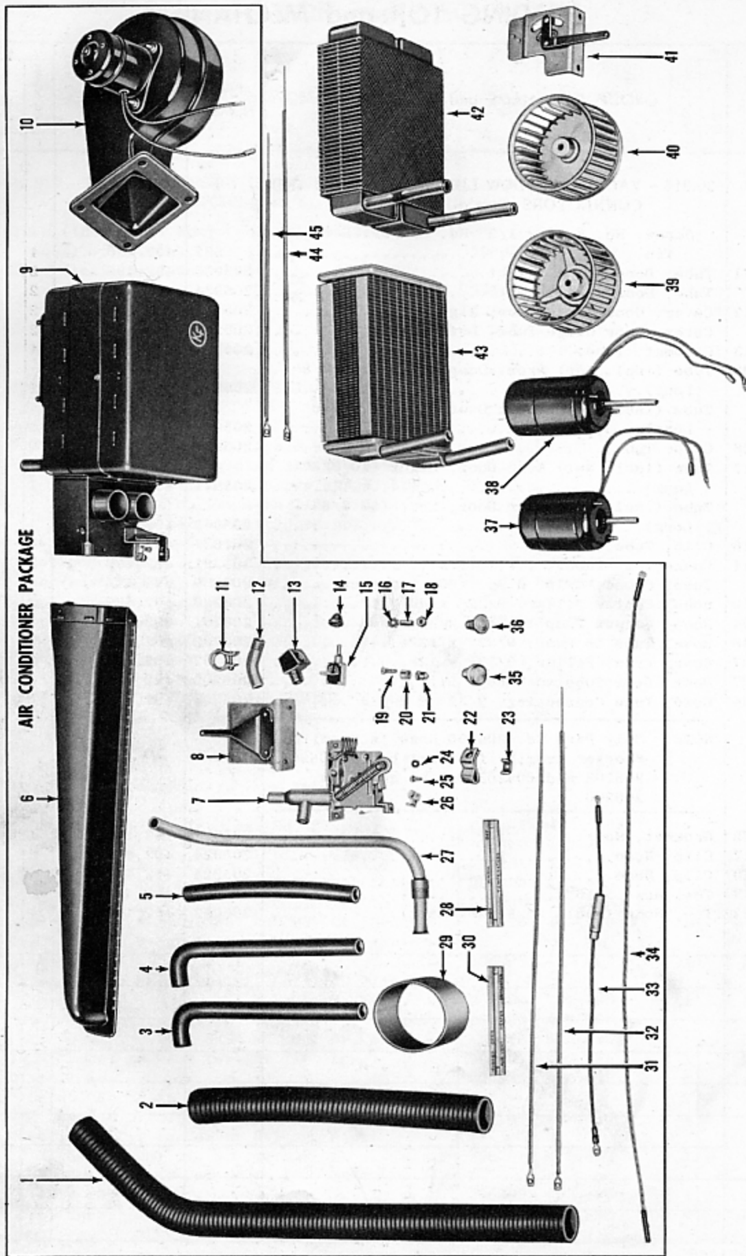
FIGURE 40-1 — AIR CONDITIONER - EXPLODED VIEW
