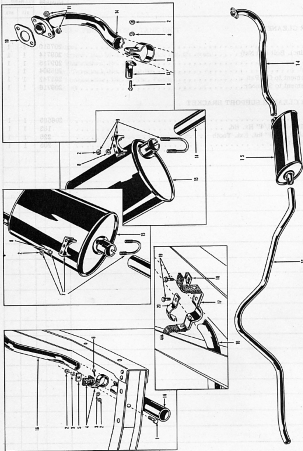
FIGURE 5-1 — EXHAUST SYSTEM
