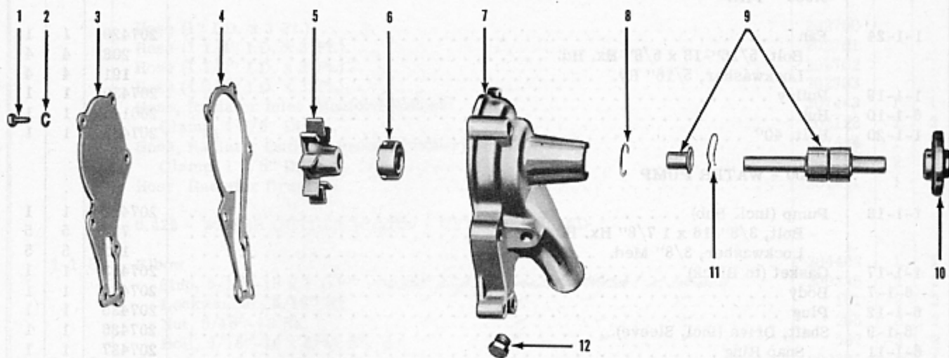
FIGURE 6-1 — WATER PUMP - EXPLODED VIEW
