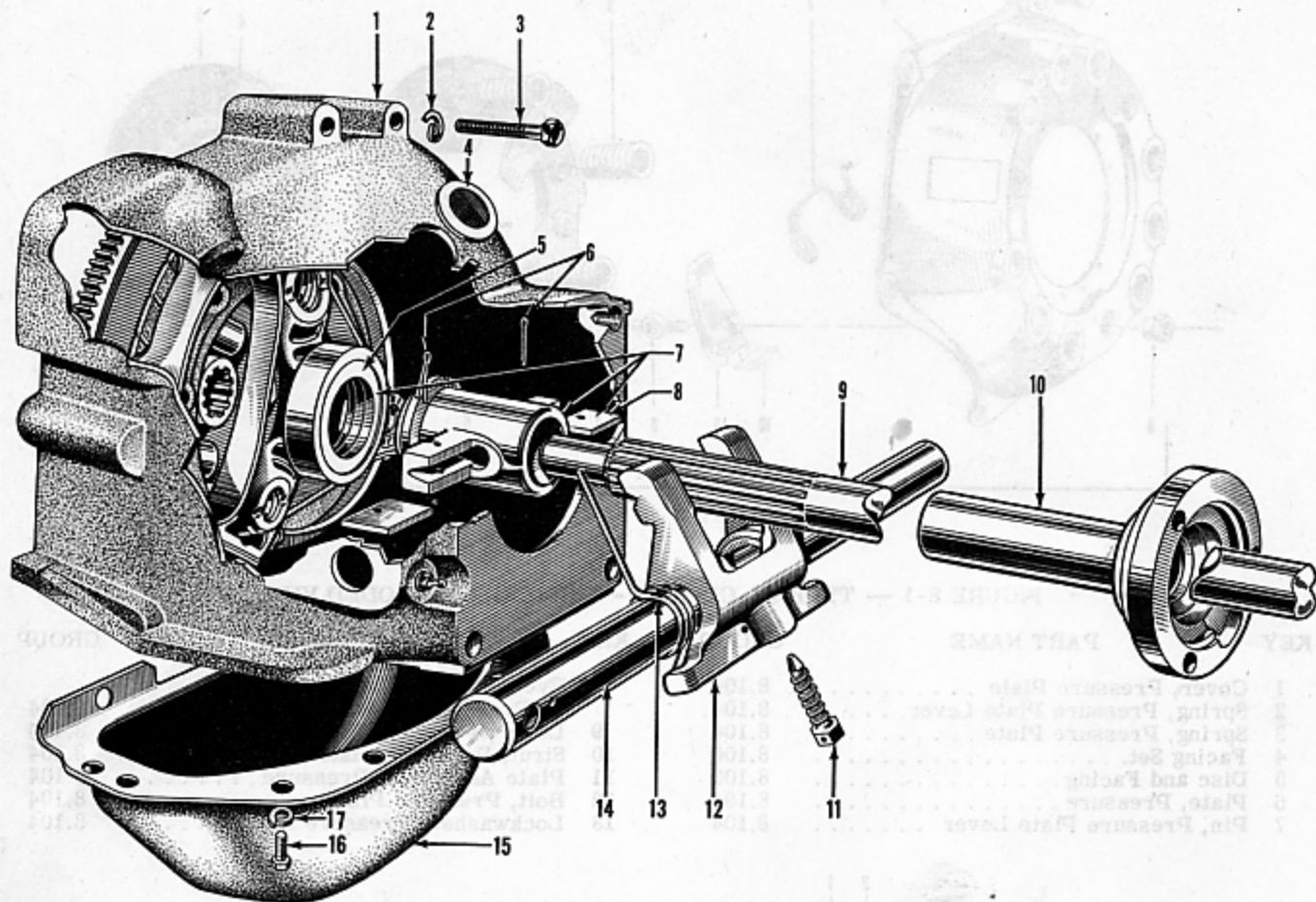
FIGURE 8-3 — CLUTCH RELEASE MECHANISM - EXPLODED VIEW
