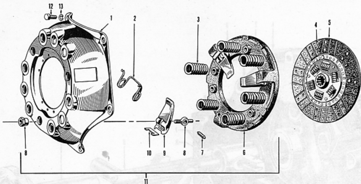
FIGURE 8-1 — TYPICAL CLUTCH - 6 SPRING - EXPLODED VIEW
