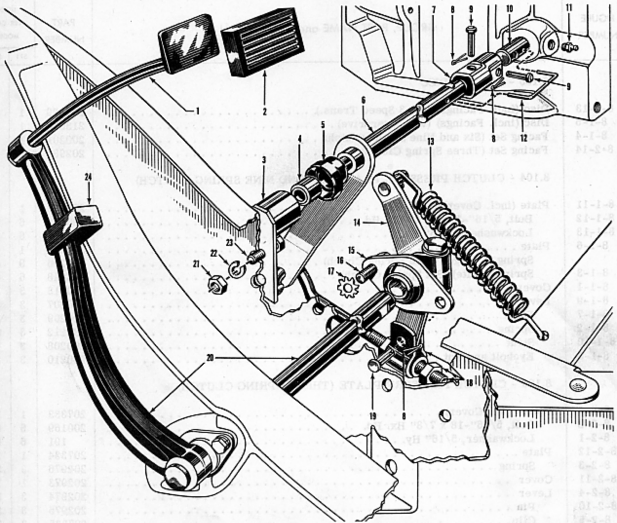
FIGURE 8-4 — TYPICAL CLUTCH LINKAGE - EXPLODED VIEW
