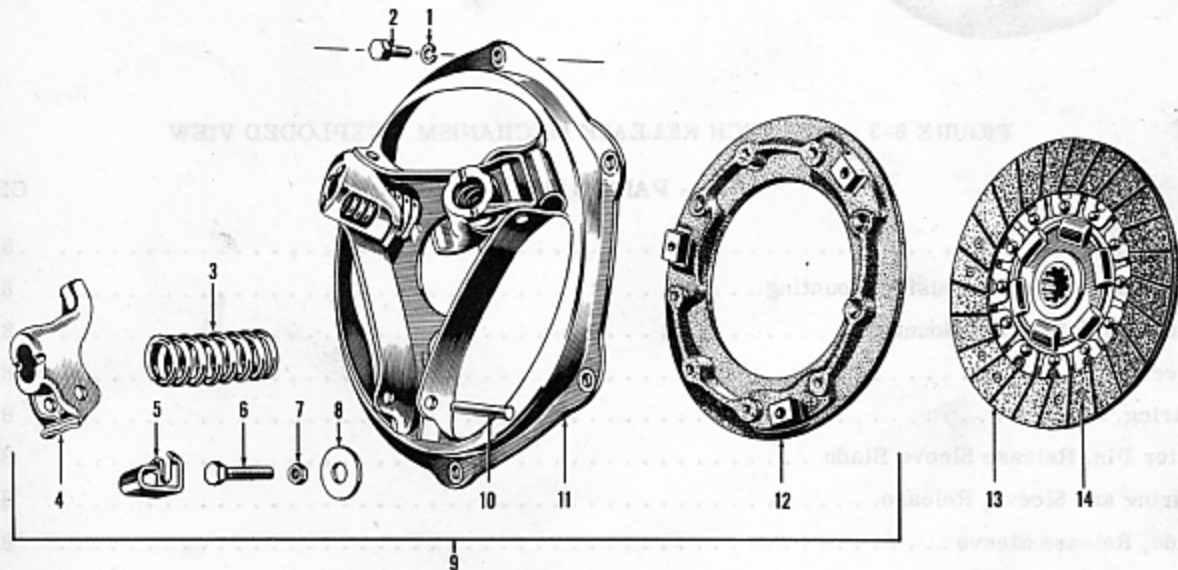
FIGURE 8-2 — TYPICAL CLUTCH - 3 SPRING - EXPLODED VIEW
