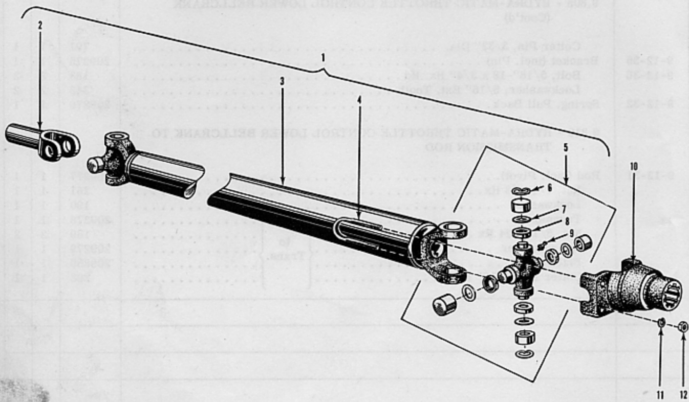
FIGURE 11-1 — TYPICAL PROPELLER SHAFT AND JOINTS - EXPLODED VIEW
