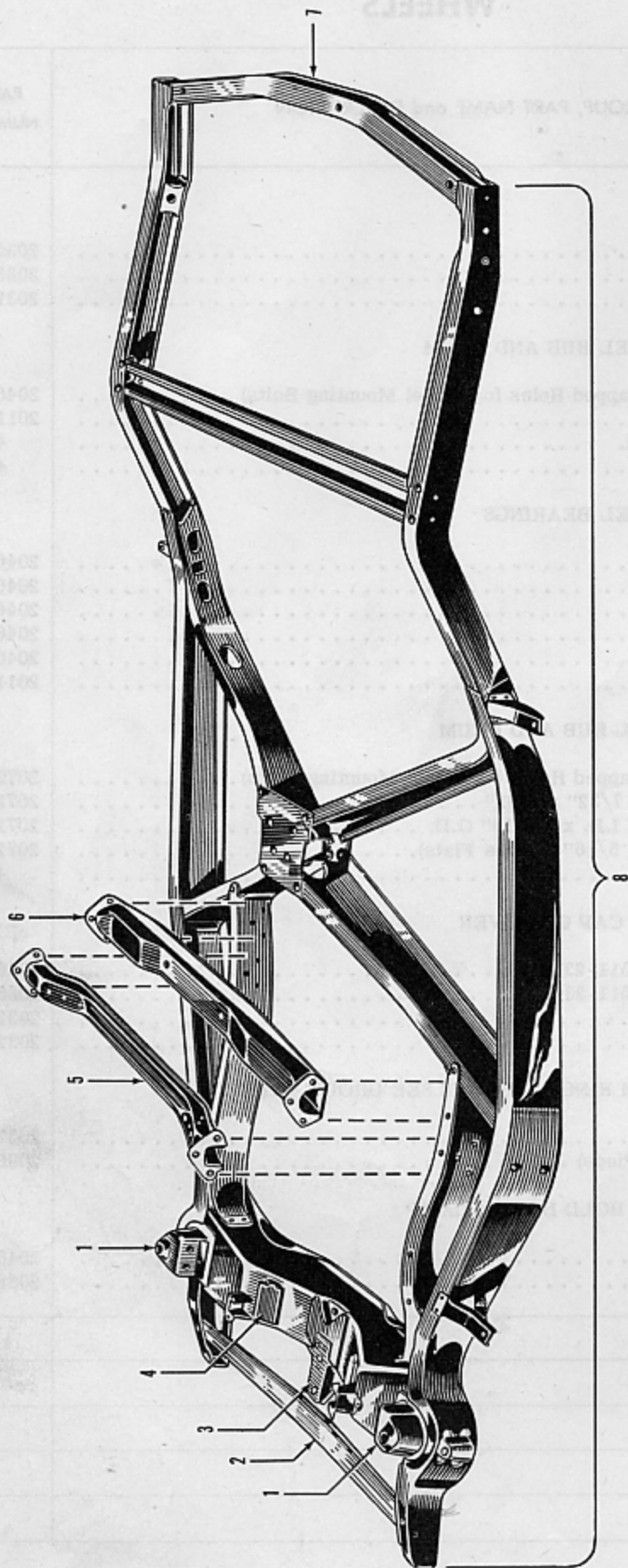
FIGURE 17-1 — FRAME ASSEMBLY
