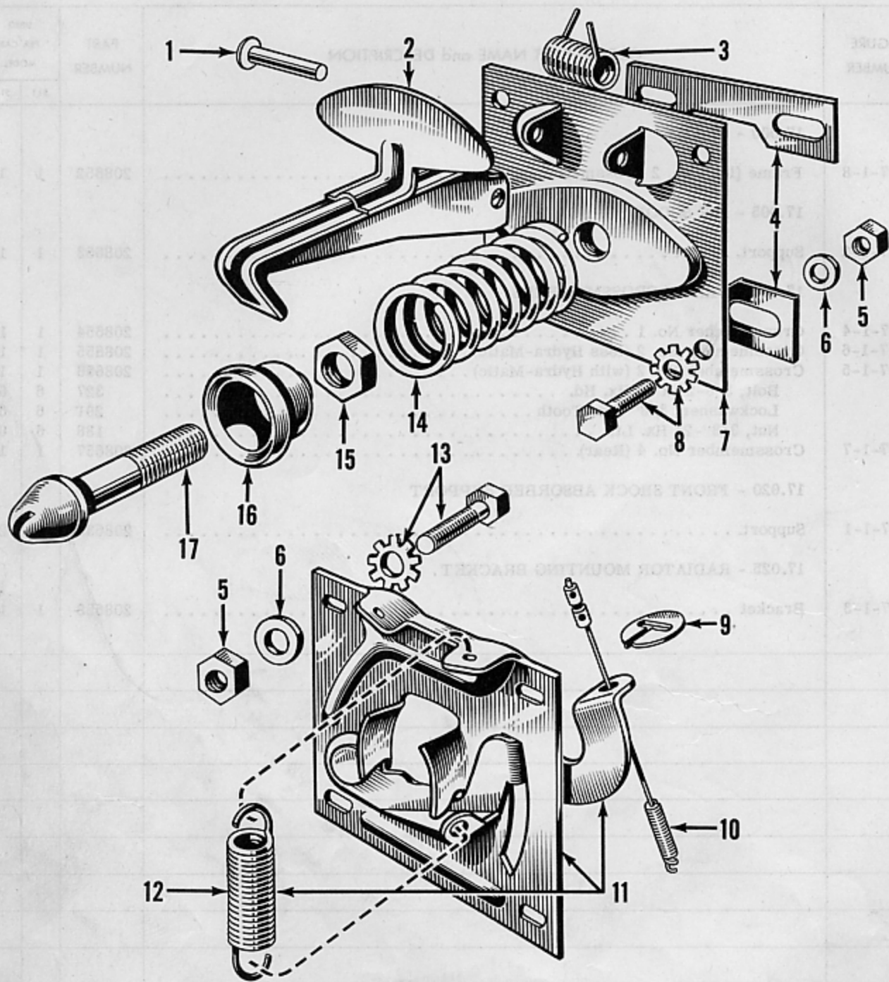
FIGURE 18-1 — HOOD LOCK MECHANISM - EXPLODED VIEW
