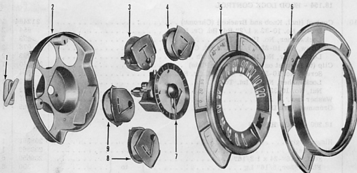
FIGURE 19-2 — INSTRUMENT CLUSTER - EXPLODED VIEW
