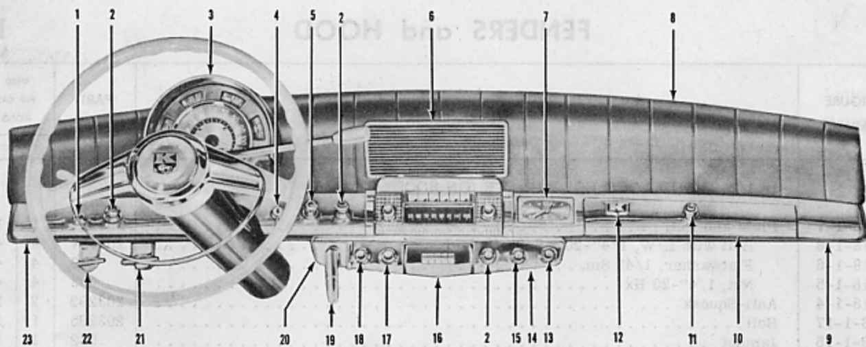
FIGURE 19-1 — INSTRUMENT PANEL
