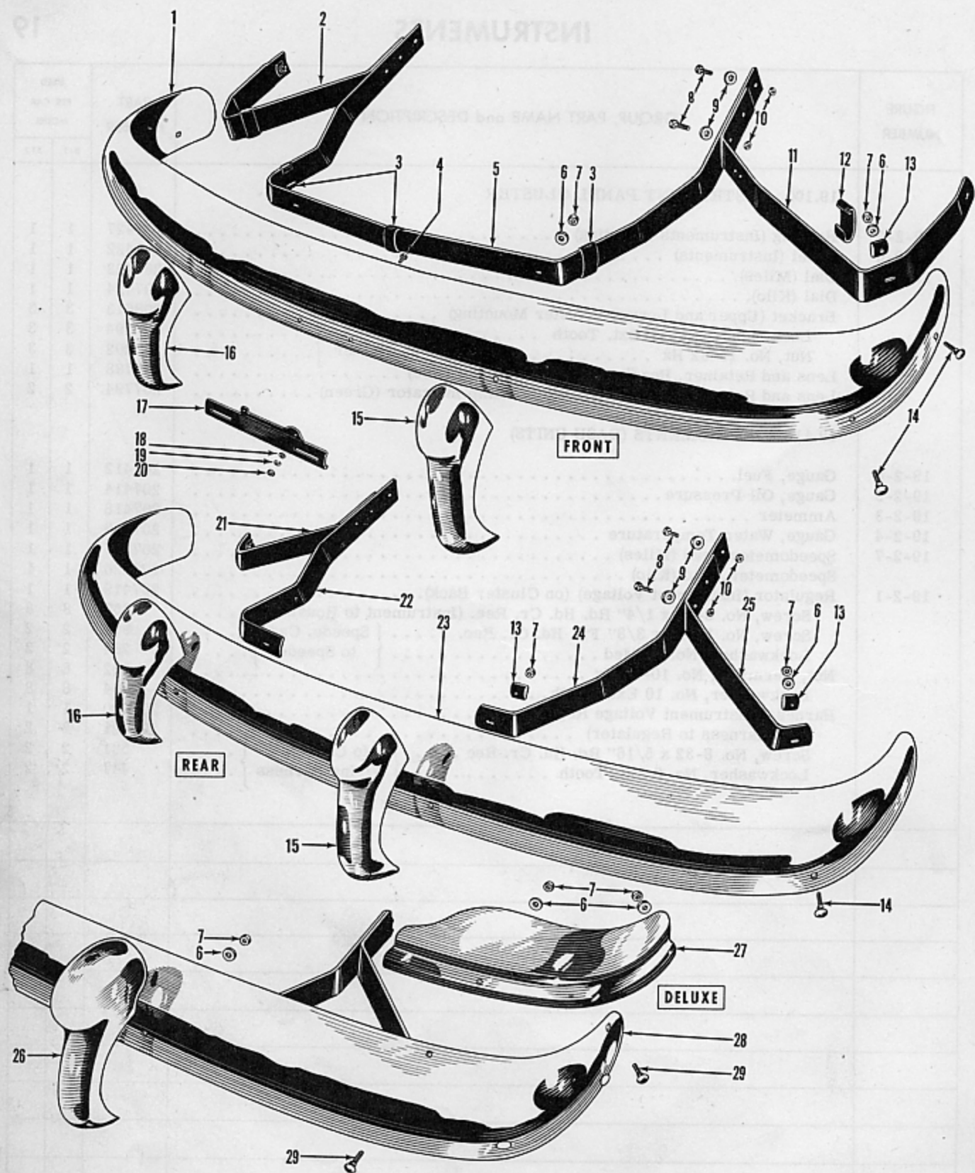
FIGURE 20-1 — BUMPERS - FRONT AND REAR - EXPLODED VIEW
