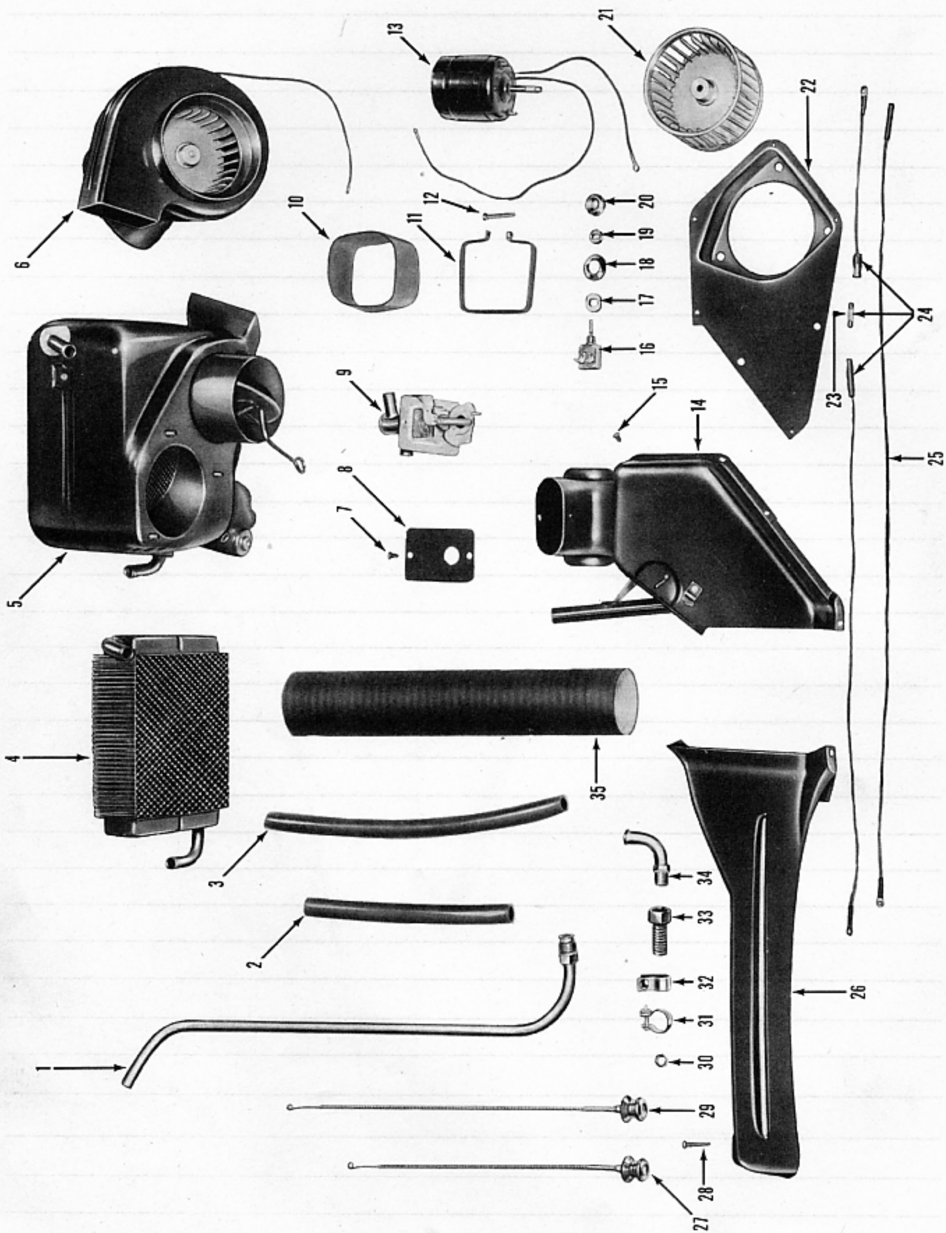
FIGURE 40-1 — AIR CONDITIONER
