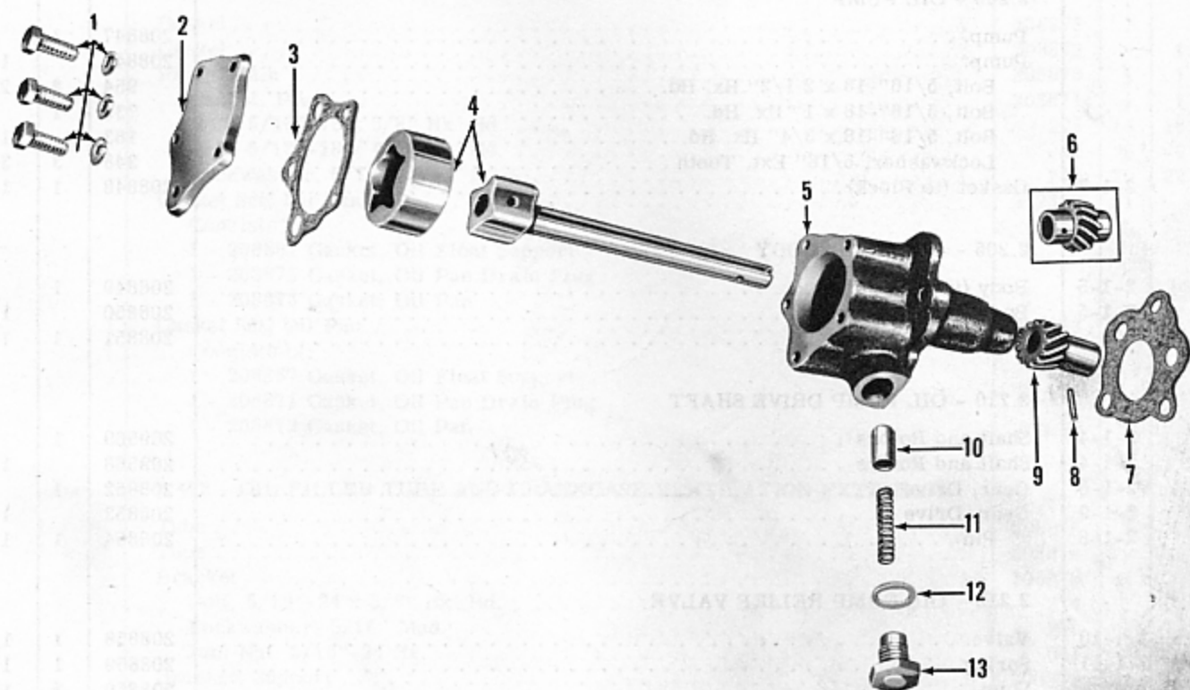
FIGURE 2-1—OIL PUMP—4 AND 6 CYLINDER—EXPLODED VIEW
