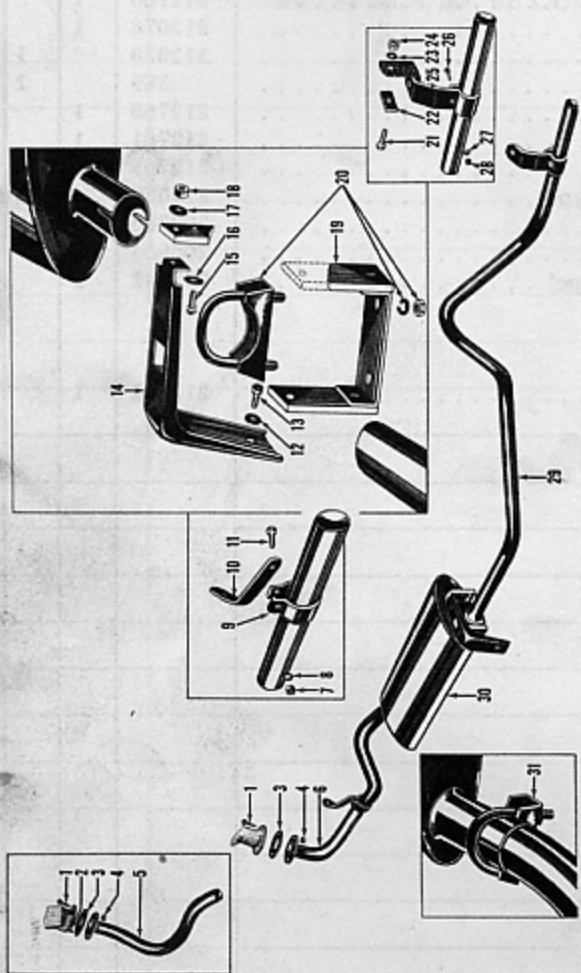
FIGURE 5-1—EXHAUST SYSTEM—4 AND 6 CYLINDER—EXPLODED VIEW
