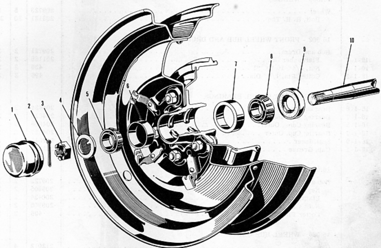
FIGURE 16-1—FRONT WHEEL AND BEARINGS—EXPLODED VIEW
