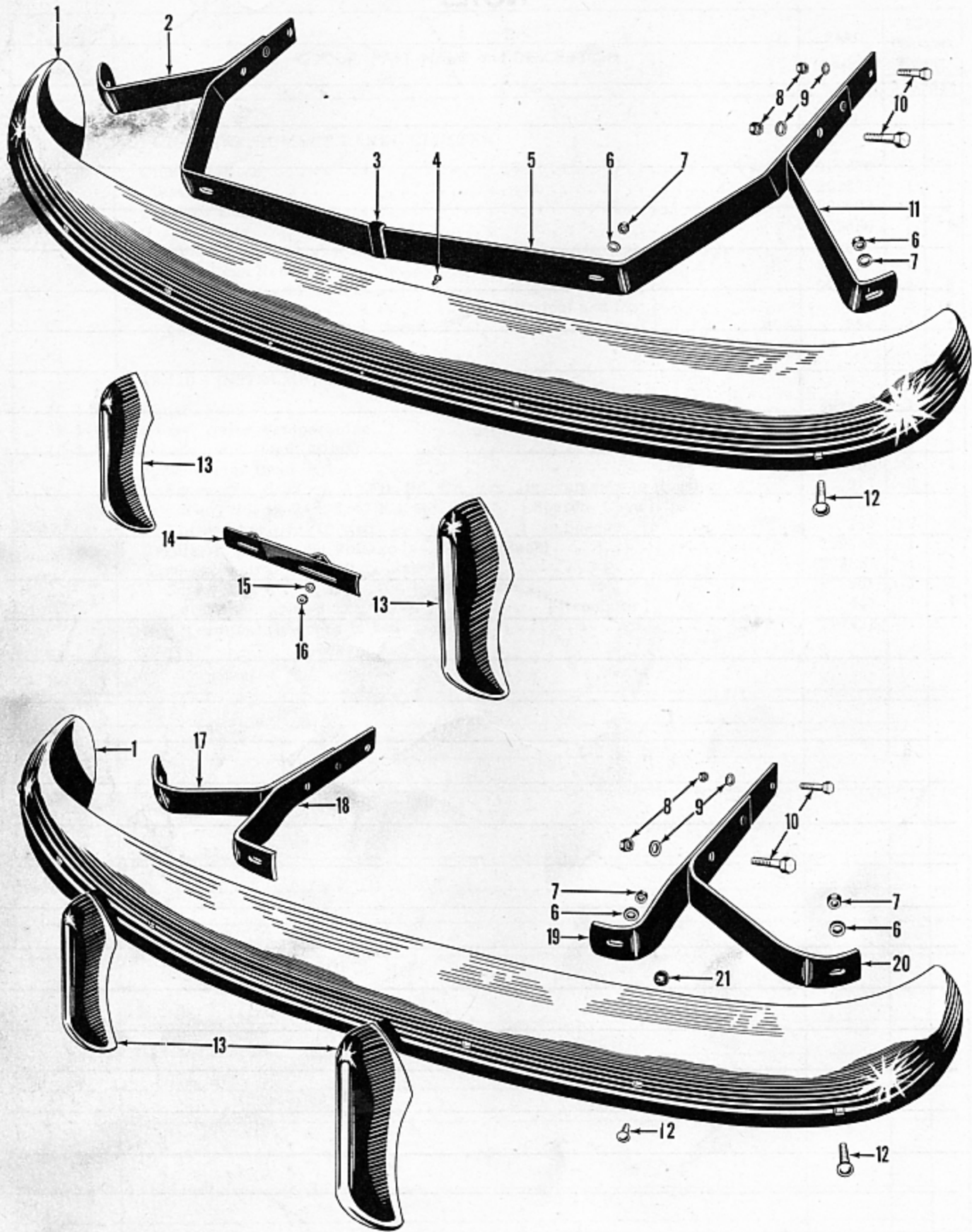
FIGURE 20-1—BUMPERS—FRONT AND REAR—EXPLODED VIEW
