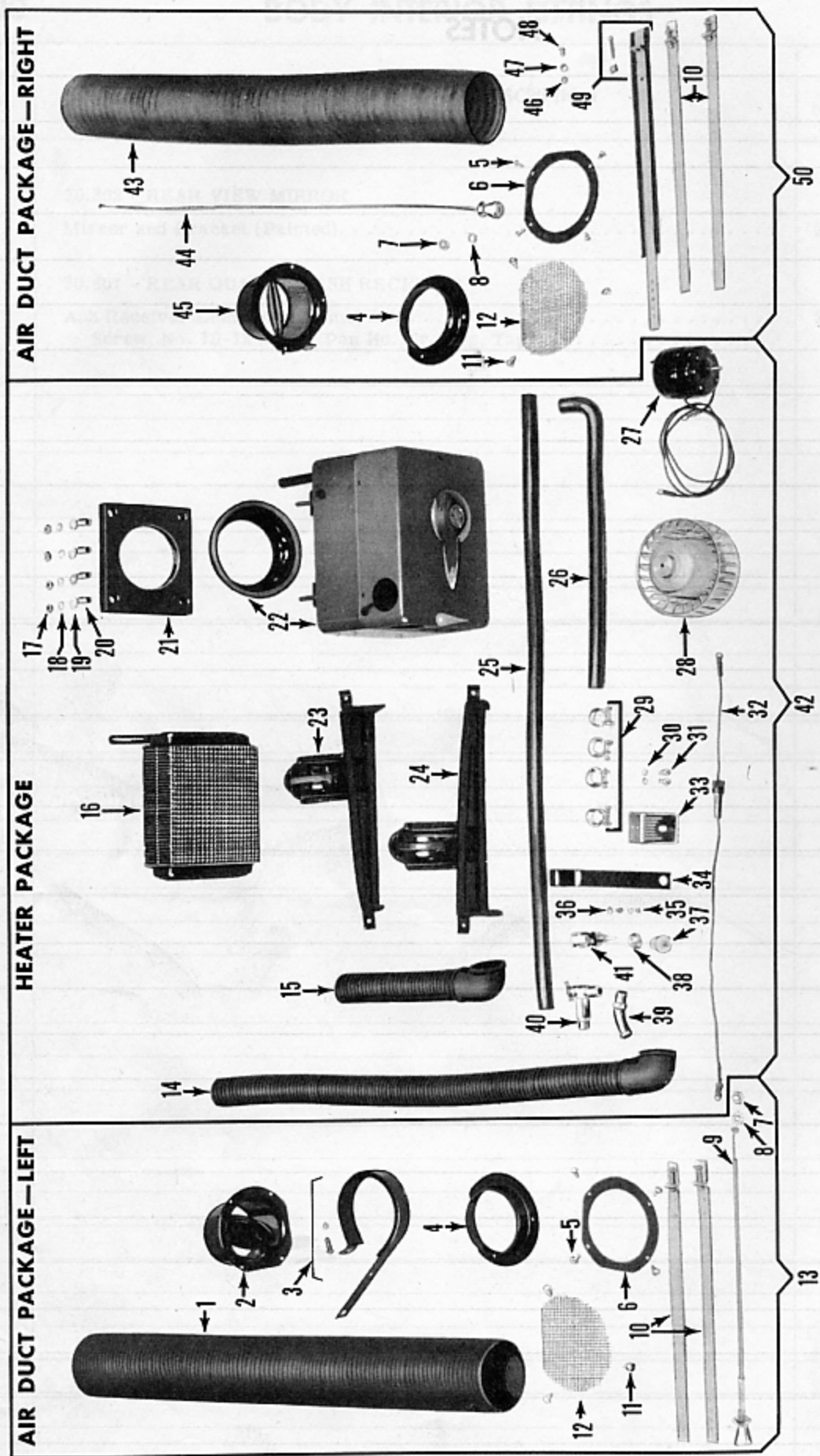
FIGURE 40-1—HEATER (Part No. 100171) AND AIR DUCTS
