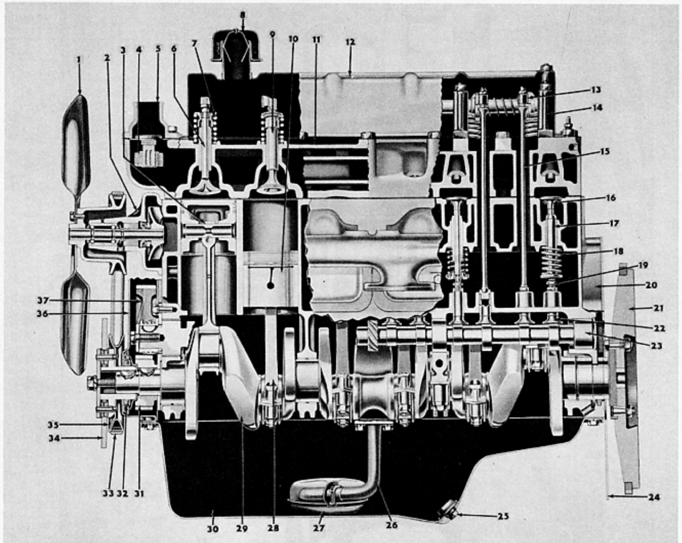
FIGURE 1-2 - SECTIONAL VIEW OF ENGINE - LEFT SIDE
