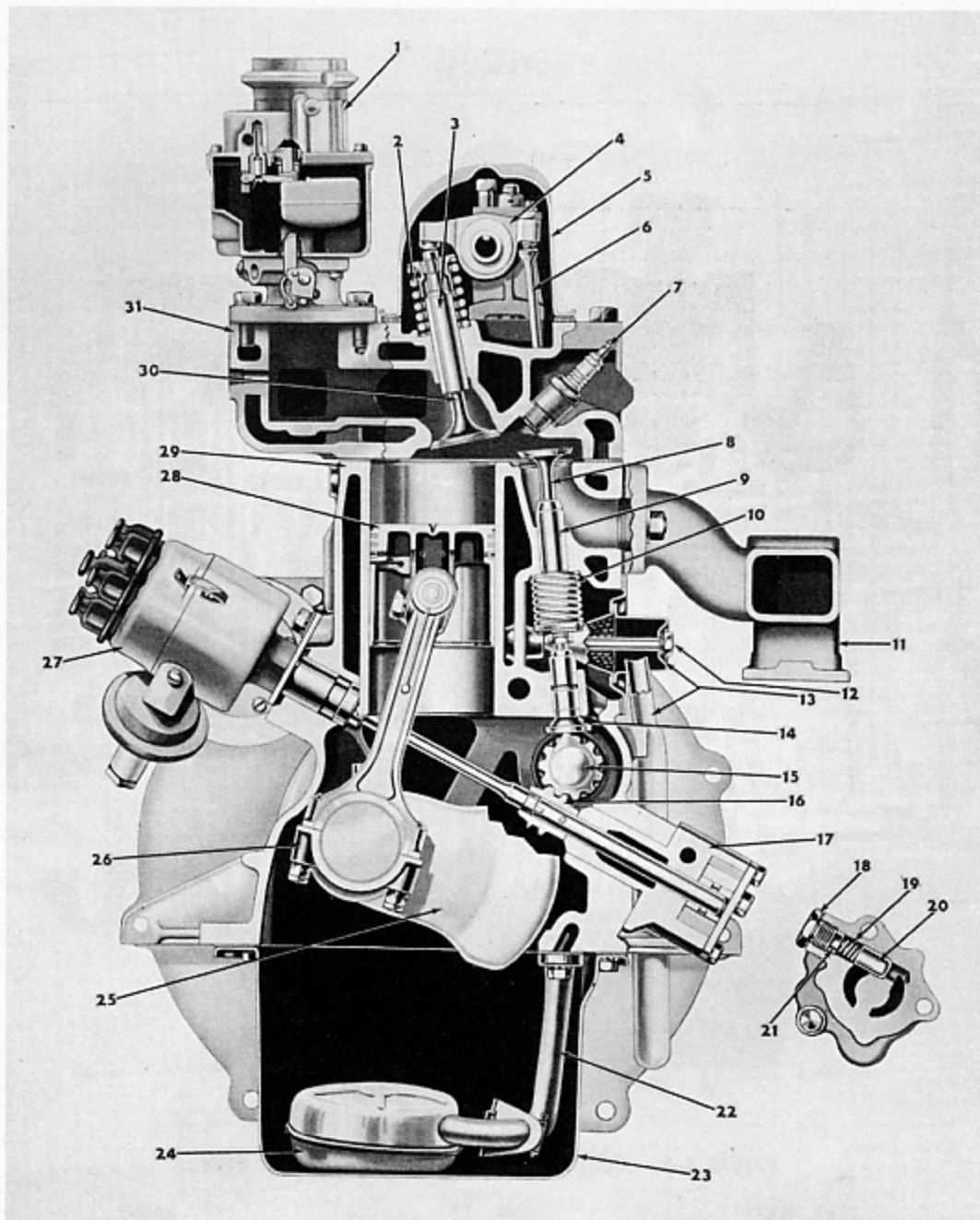
FIGURE 1-3 - SECTIONAL VIEW OF ENGINE - FRONT
