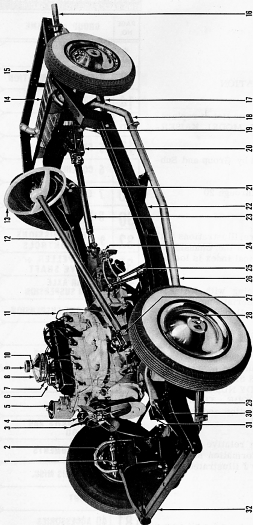
FIGURE 1-1 - CHASSIS
