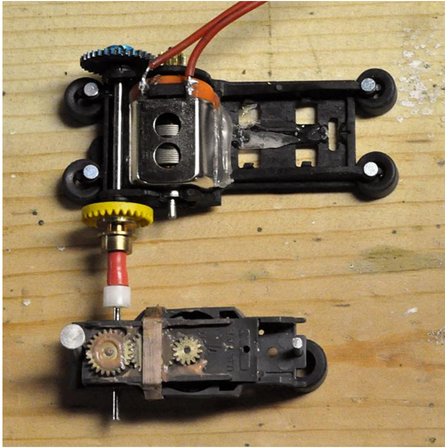
Gear lapping rig
